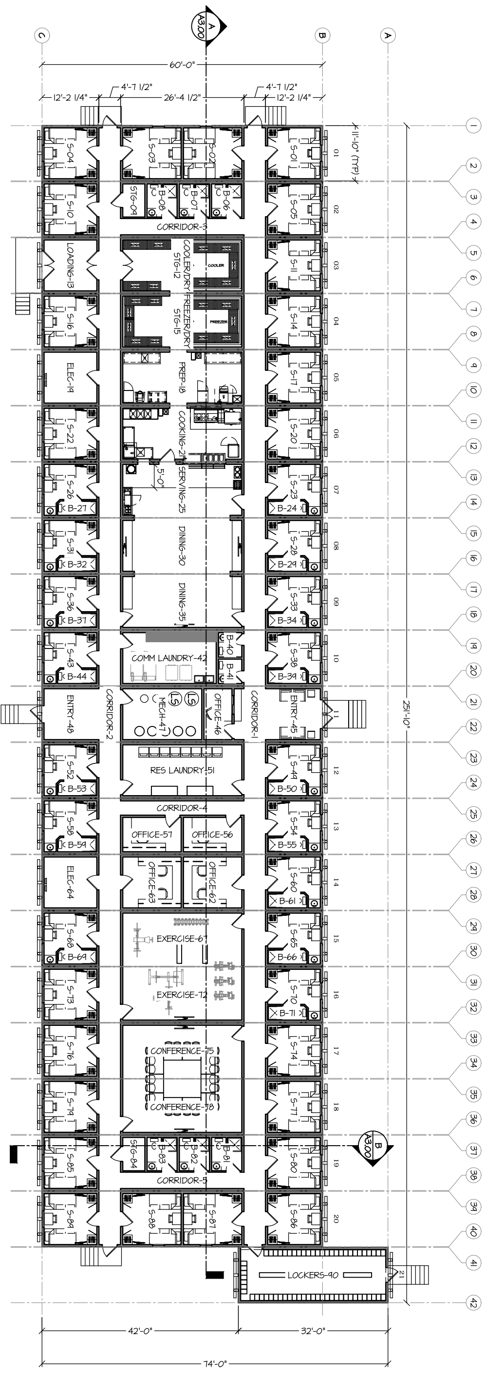
OVERALL PLAN 1/20" = 1'-0"
